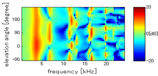
Figure 10. HRTFs for “1/3 position model.”
